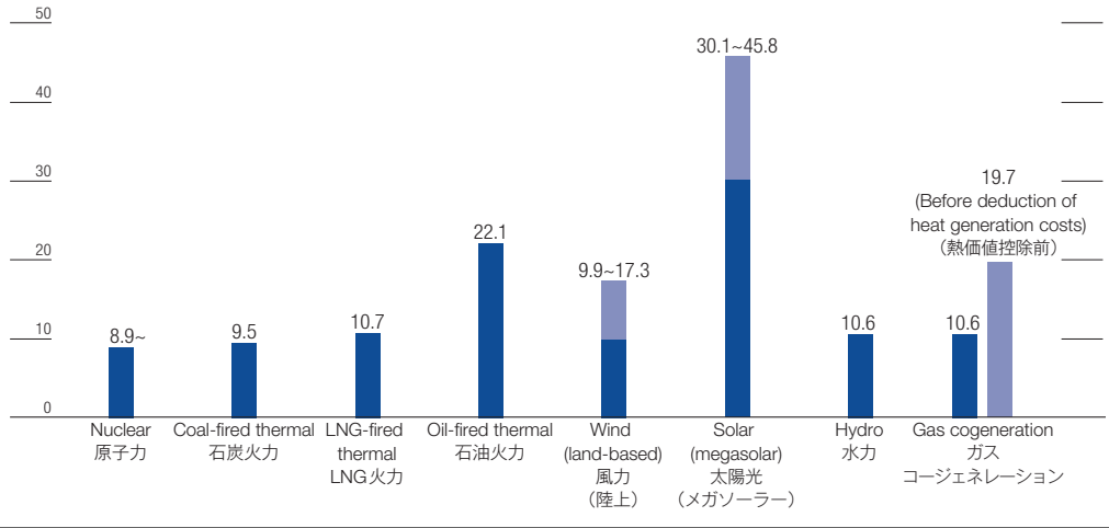
Generation Costs by Power Source (2010 Model Plants) (Yen/kWh)
